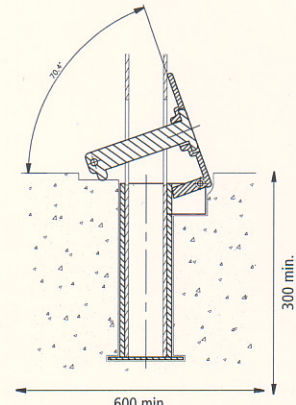
PORTABLE INGROUND FOOTING
