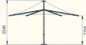
5.6m HEXAGONAL
