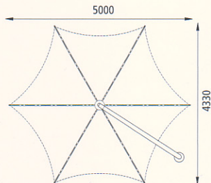
5.0m HEXAGONAL CANTILEVER
