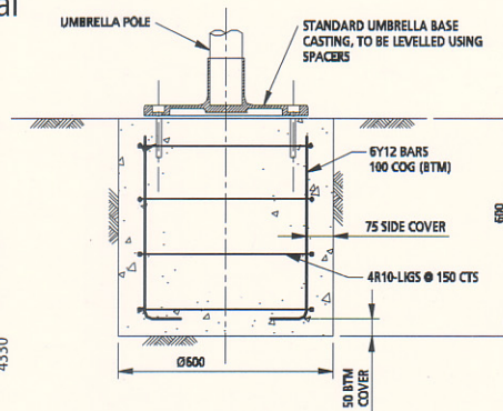
STATIC UMBRELLA FOOTING
