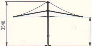
4.0m SQUARE
