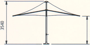
3.5m SQUARE
